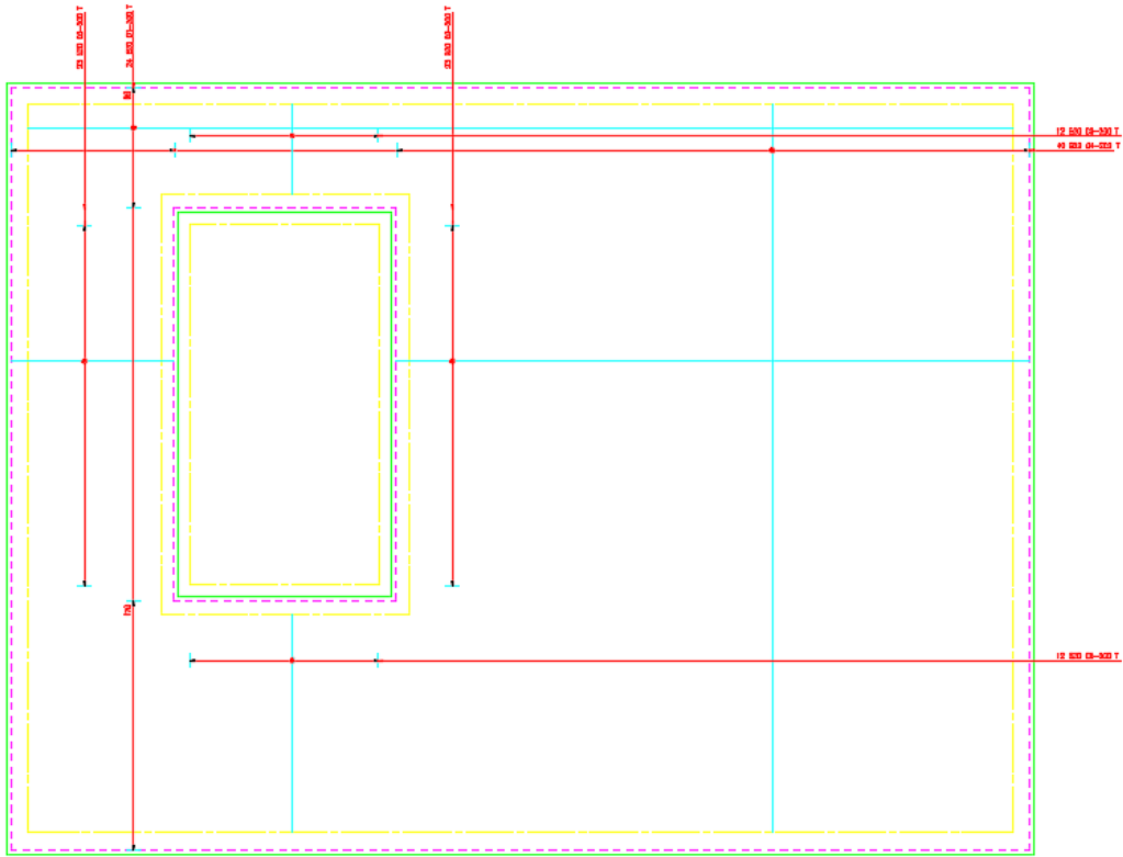
Figure 1.15 Drawing showing top steel only
