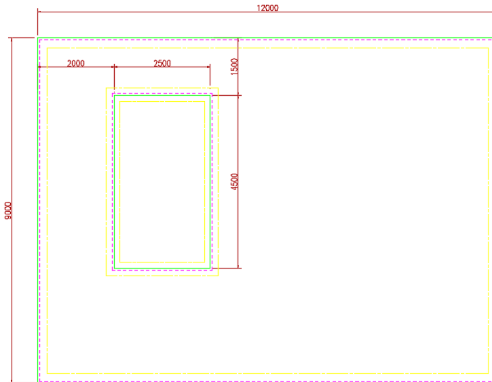
Figure 1.6 General Arrangement Drawing
