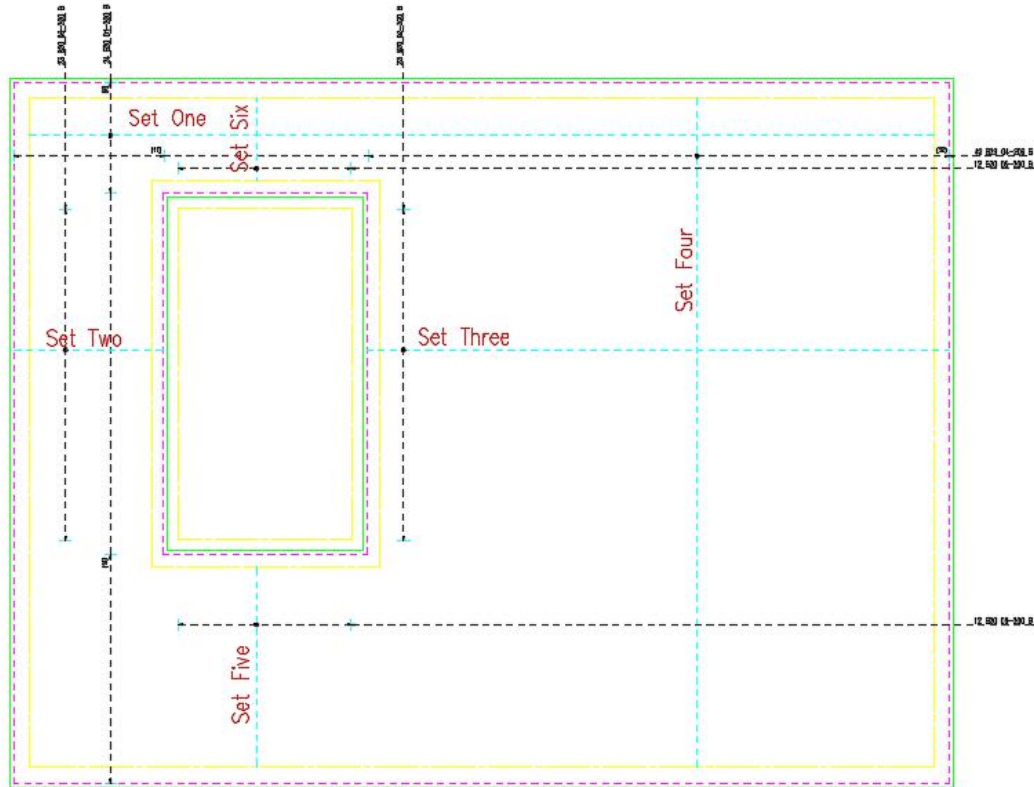
Figure 1.8 Reinforcement drawing showing bottom steel
