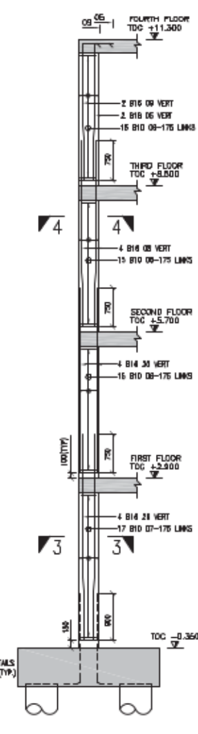
ELEVATION OF COLUMN B1 SCALE 1:50 SIZE: 400x400 (2 NO. THRS)
