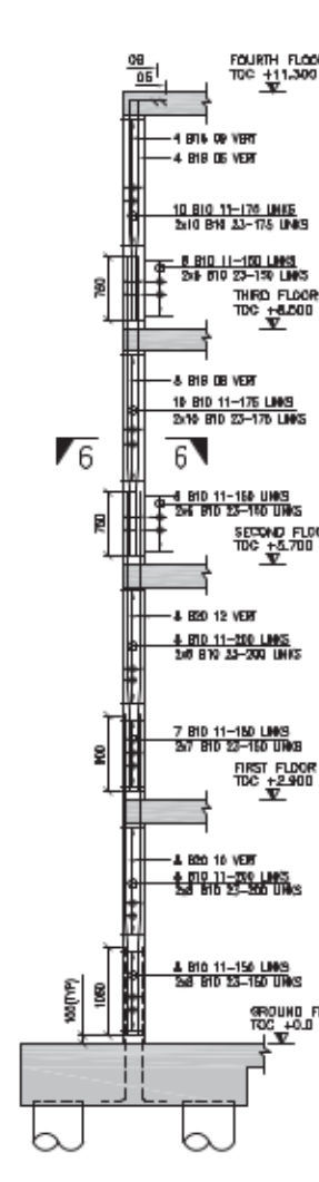
ELEVATION OF COLUMN C SCALE 1:50 SIZE: 200x200
