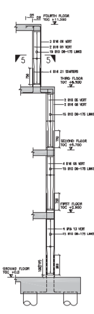
ELEVATION OF COLUMN D2 SCALE 1:50 SIZE: 400x400 (3 NO. THRS)
