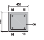
SECTION 8-8 SCALE 1:20
