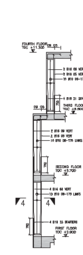
ELEVATION OF COLUMN D4 SCALE 1:50 SIZE: 400x400
