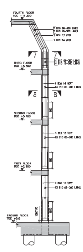
ELEVATION OF COLUMN G SCALE 1:50 SIZE: 400x400
