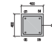
SECTION 5-5 SCALE 1:20
