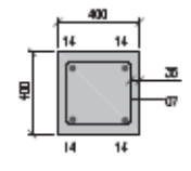
SECTION 9-9 SCALE 1:20
