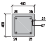
SECTION 3-3 SCALE 1:20
