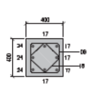
SECTION 7-7 SCALE 1:20
