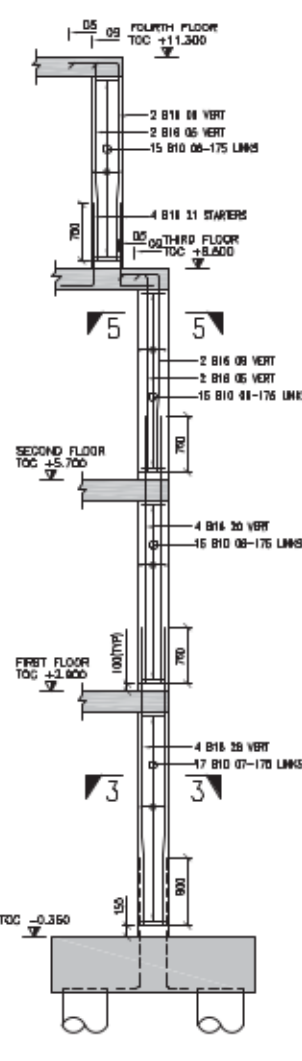
ELEVATION OF COLUMN B2 SCALE 1:50 SIZE: 400x400 (2 NO. THRS)
