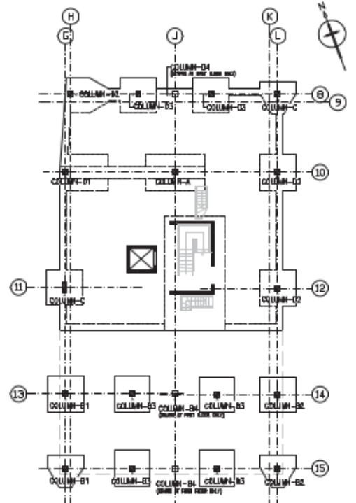
GROUND FLOOR KEY PLAN (BLOCK - B) RTS
