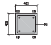
SECTION 4-4 SCALE 1:20
