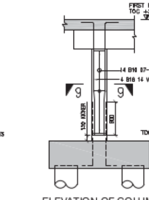
ELEVATION OF COLUMN B3 SCALE 1:50 SIZE: 400x400 (4 NO. THRS)
