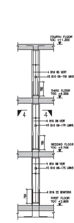
ELEVATION OF COLUMN B4 SCALE 1:50 SIZE: 400x400 (2 NO. THRS)
