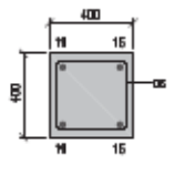
SECTION 10-10 SCALE 1:20
